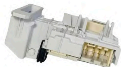
W10707441 LOCK - LID, TOP, SOLENOID, LIGHT GRAY Switch Tapa W10707442
