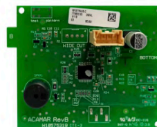
W10776435 EXTERNAL UI B_1 FOR JAGUAR II AGITATOR Tarjeta Interface
