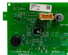
W10788857 EXTERNAL UI FOR JAGUAR IMPELLER B Tarjeta Interface
